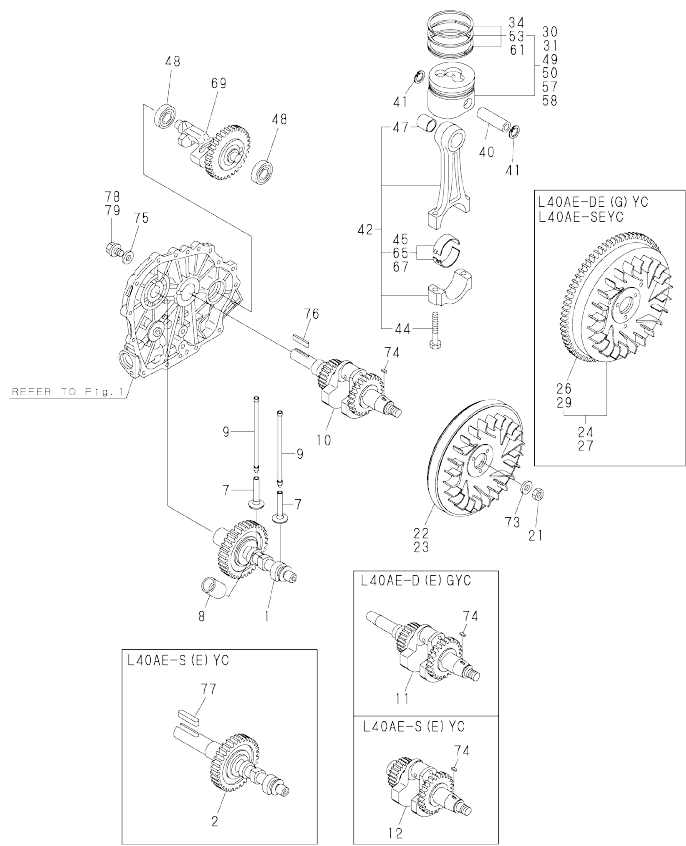
Fig.4. CRANKSHAFT,PISTON & CAMSHAFT
